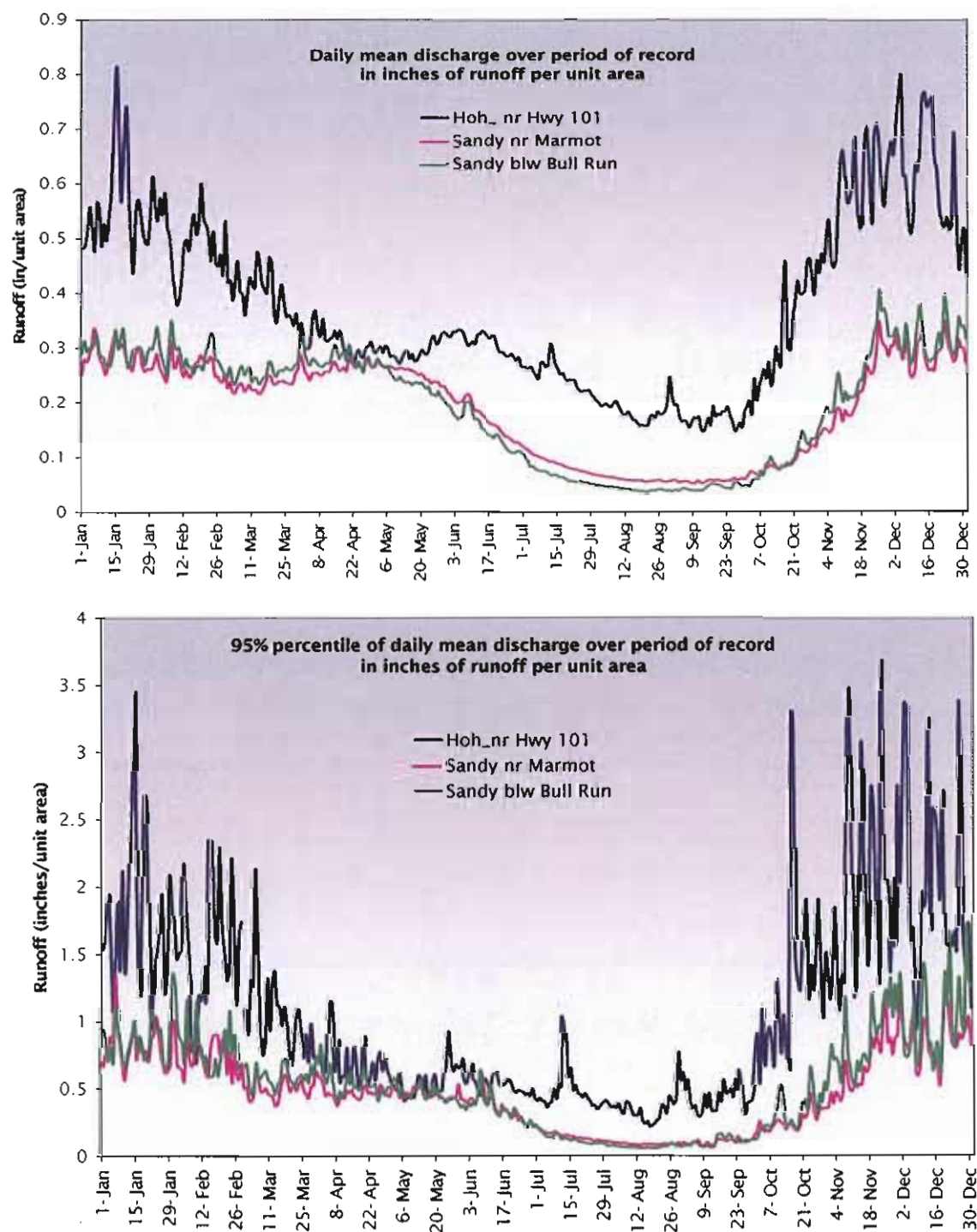
Figure 1: Hydrographs of a) mean daily and b) 95% percentile of the mean daily discharge, normalized as runoff in inches per unit area for comparison, illustrate the difference in discharge between the Hoh and Sandy River. Runoff to the Hoh is much greater and more variable with greater transport capacity throughout the year. This example illustrates short-comings of using very different river systems as examples of what can be done on the Hoh. Such comparisons can lead to the “bad and ugly” not “good” solutions.
