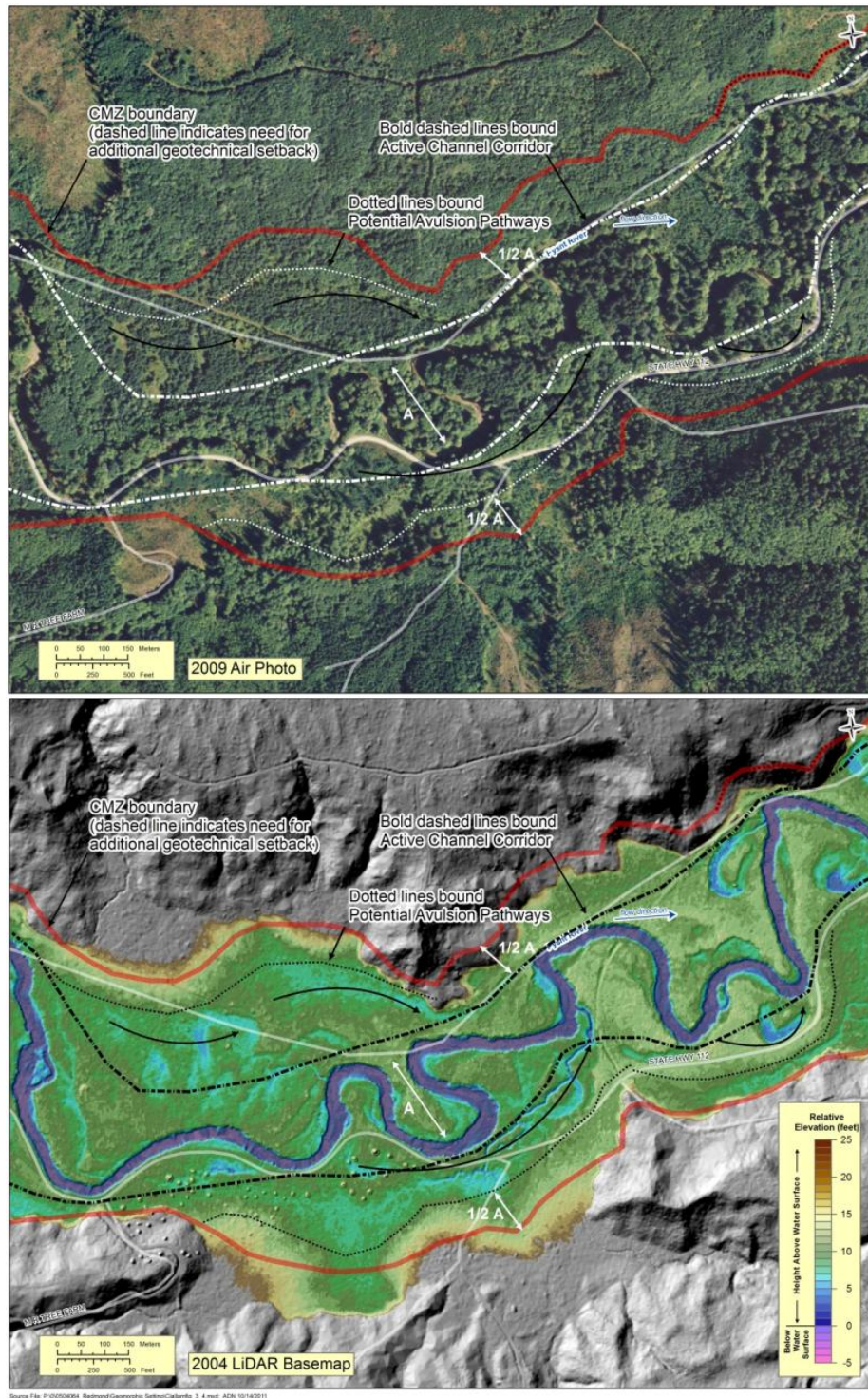
Figure 4.4: Aerial image (above) and RWSE map (below) for Pysht River showing the Active Channel Corridor, potential avulsion pathways, and channel migration buffer.
