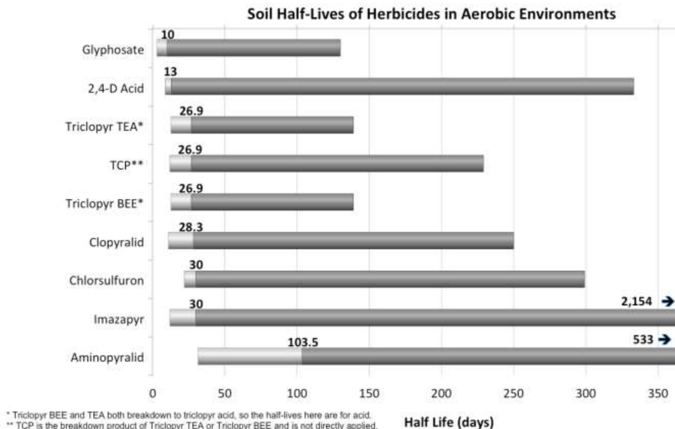
Figure 4: Comparison of the range of herbicide half-lives under aerobic conditions in soil. The high end of the range is typically under arid conditions where microbial degradation rates are low. Exposure to sunlight can accelerate decomposition and shorten the half-life of some herbicides. Sources are described after Table 12. For aminopyralid, see EPA Fact Sheet 2005 . For imazapyr, see EPA 2007 Appendix A Imazapyr Effects Determination for the CA Red-legged frog .
